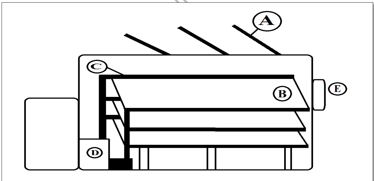
316 Figure 4- It's a basic design of Eco-Friendly Soilless Farming Unit (EFSFU) where A ; solar 317 panels, B ; culture racks, C ; nutrient supplying system, D ; control panel, E ; air circulation 318 system. The front entrance has extra chamber to keep all sterilized tools, equipments and 319 clothing.
