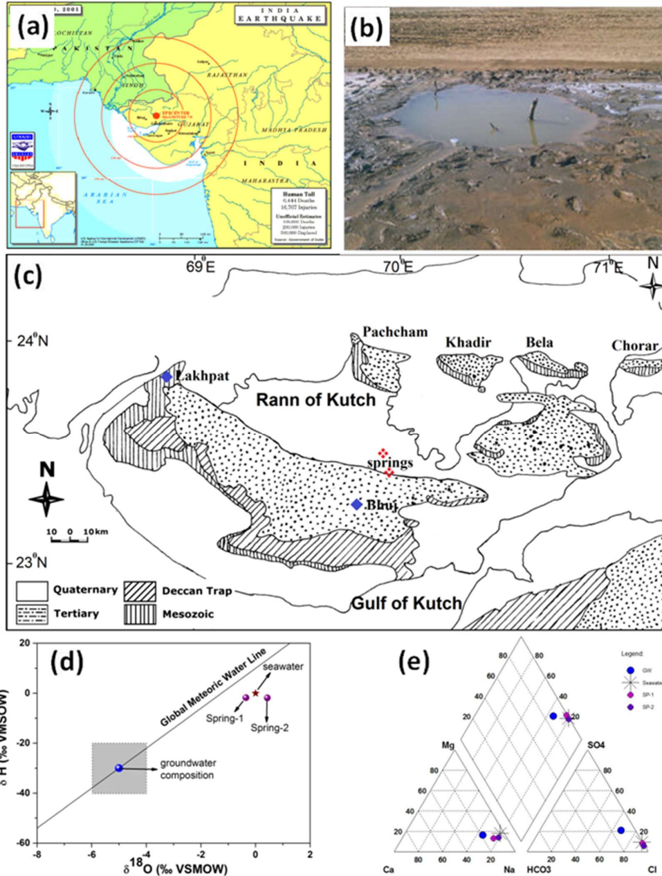
Figure 1 a) Epicentre of the earthquake 5 , b) Springs emerged after the event 5 , c) location of the springs, d) isotopic identification of spring water source and ground waters of present day, the shaded portion indicates the extent of isotopic variation and e) Piper's trilinear plot of the major ion data of springs (shown by red and purple circles), local groundwater (shown by blue circle) and seawater (shown by asterisk).
