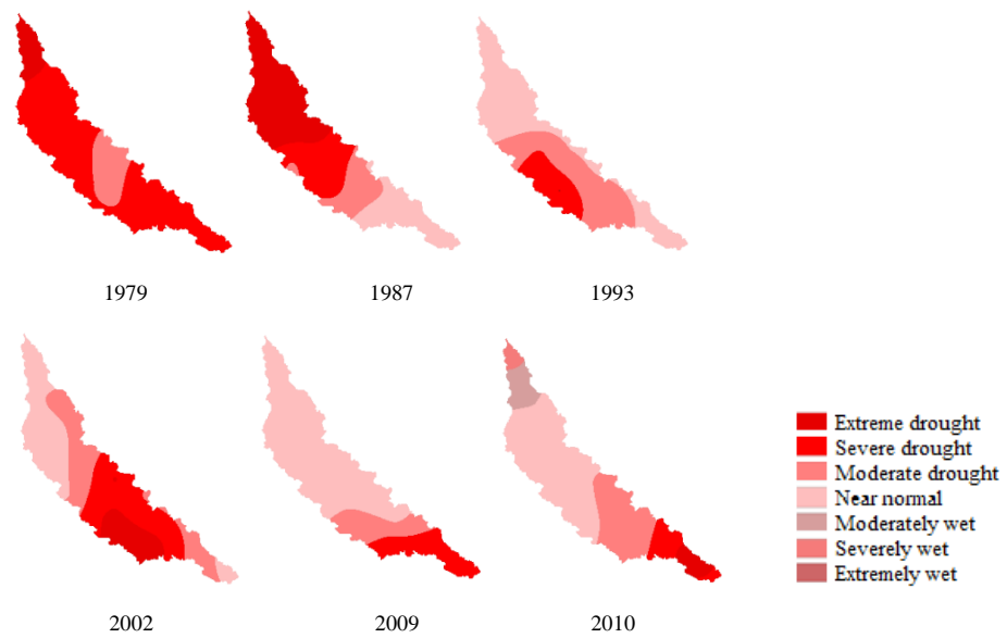
Figure 4. June-September 4-month SPI for Gomti basin
