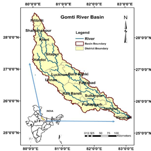
Figure 1. Location of the Gomti river basin in India 25
