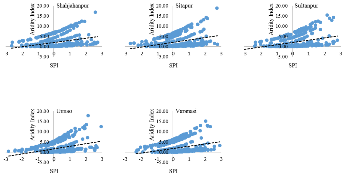
Figure 5. Scatter plots and correlation lines between de Martonne aridity index and SPI for all districts of Gomti basin
