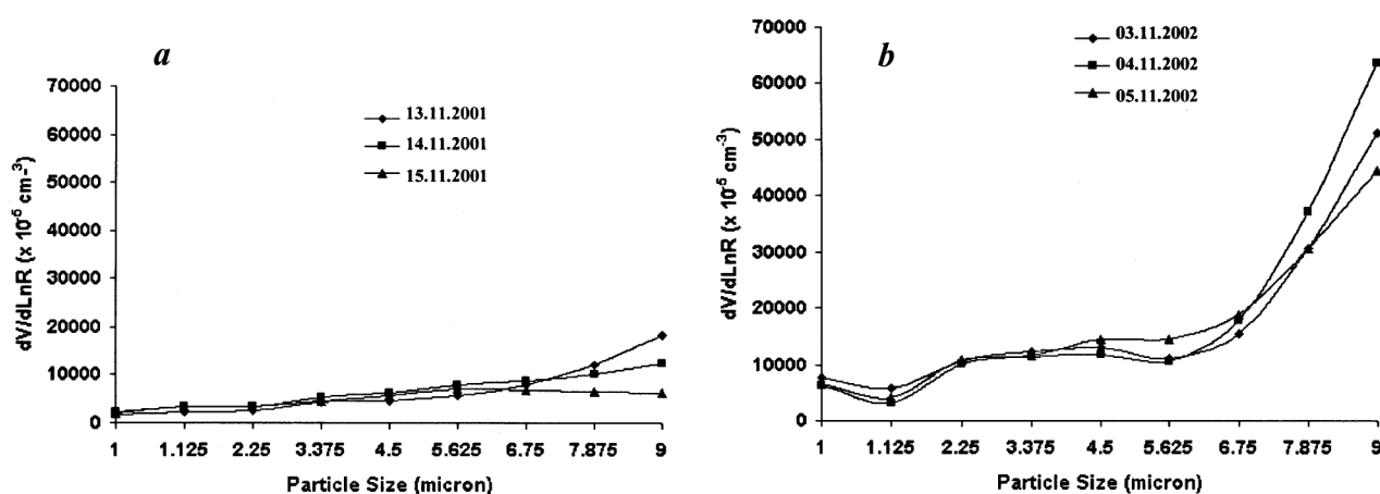
Figure 3. Size distribution of super-micron aerosols during Diwali festival of the year (a) 2001; (b) 2002.
