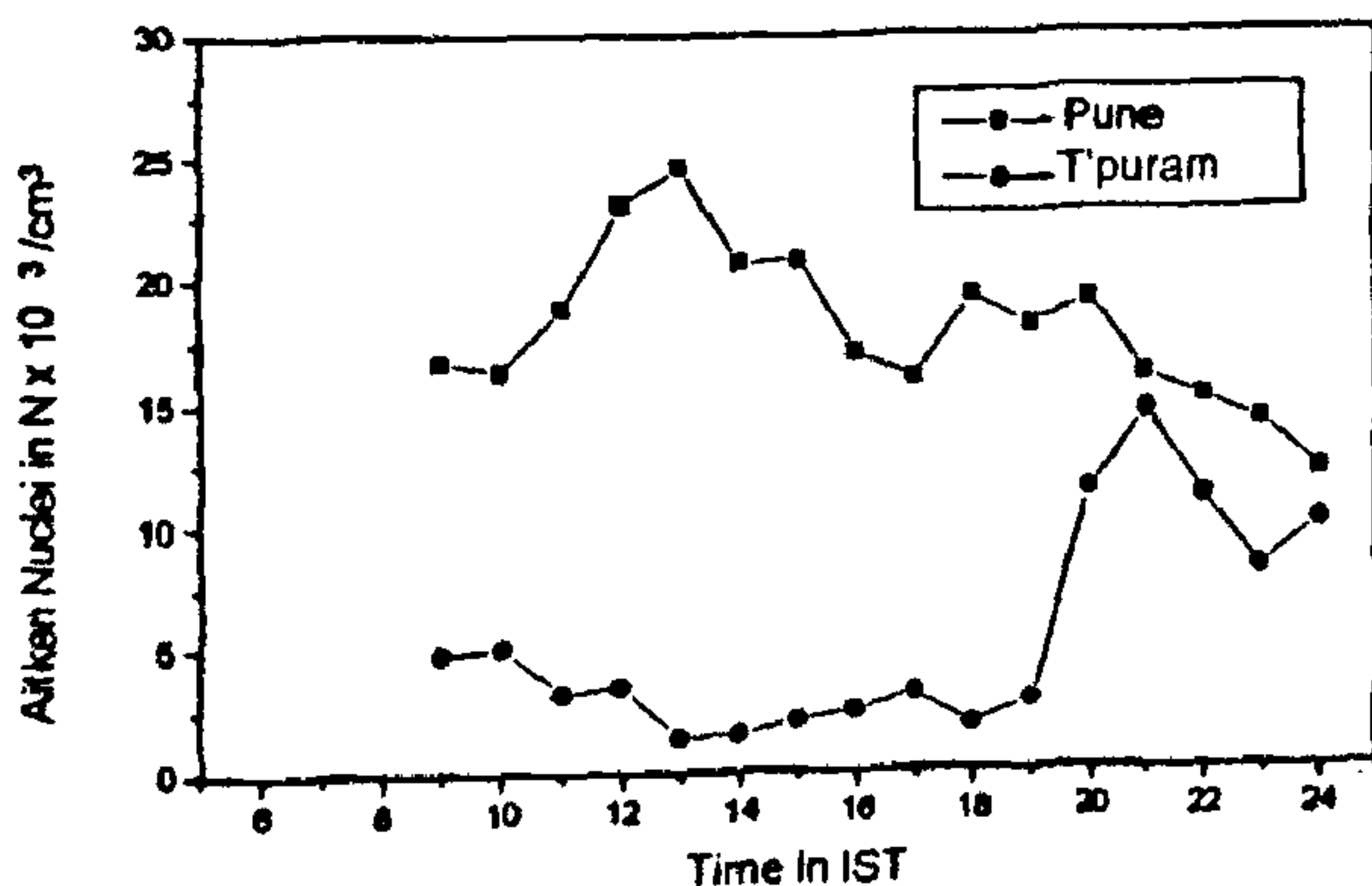
Figure 1. Diurnal variation of Aitken nuclei at Pune and Thiruvananthapuram.
