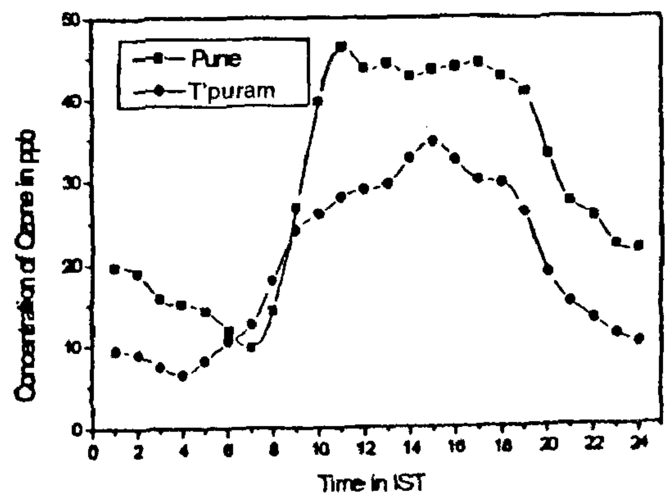
Figure 2. Diurnal variation of ozone at Pune and Thiruvananthapuram.
