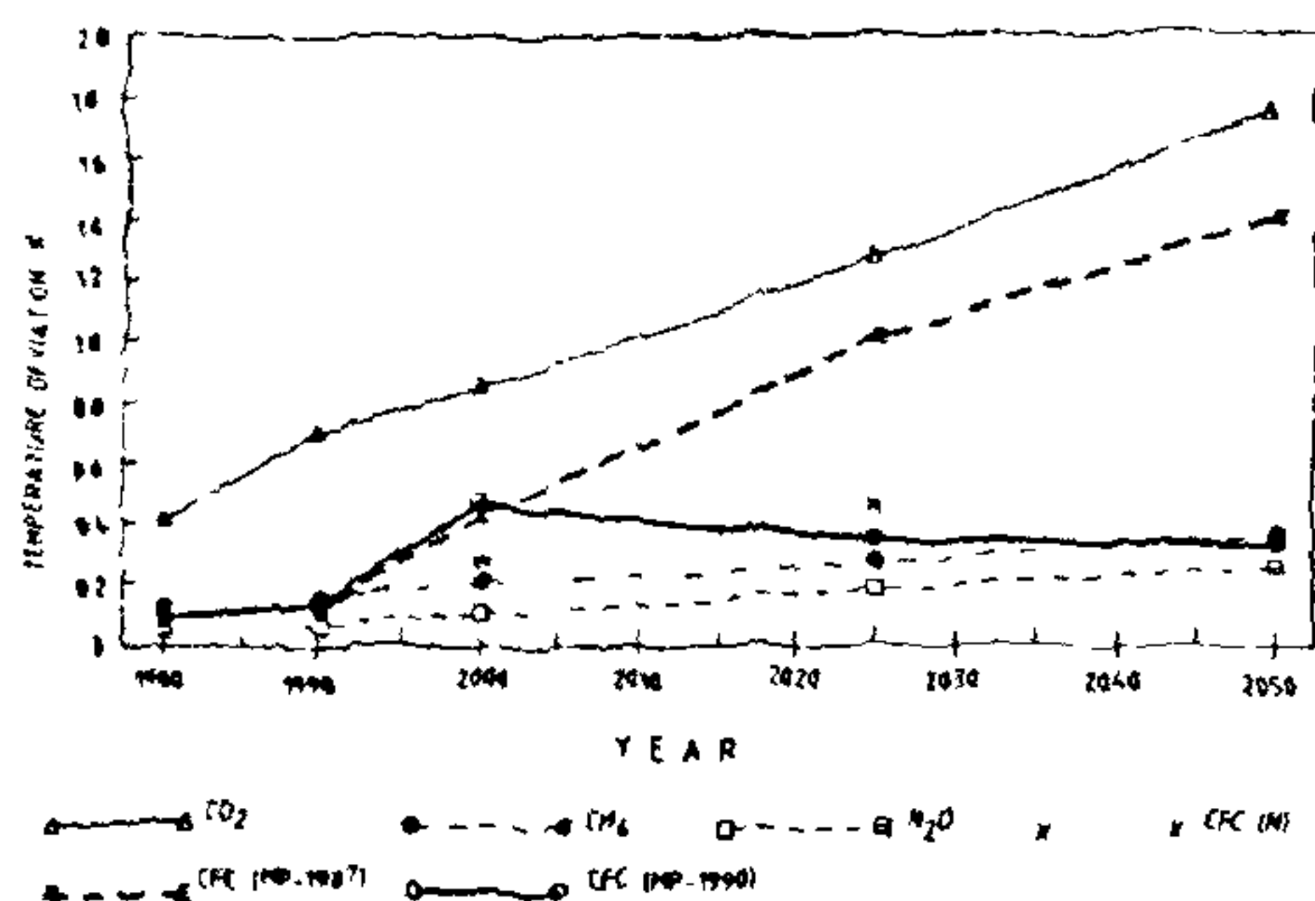
Figure 4. Global change in temperature calculated using the Energy Balance model for the projected atmospheric concentrations of greenhouse gases shown in Figure 2 and Figure 3.
