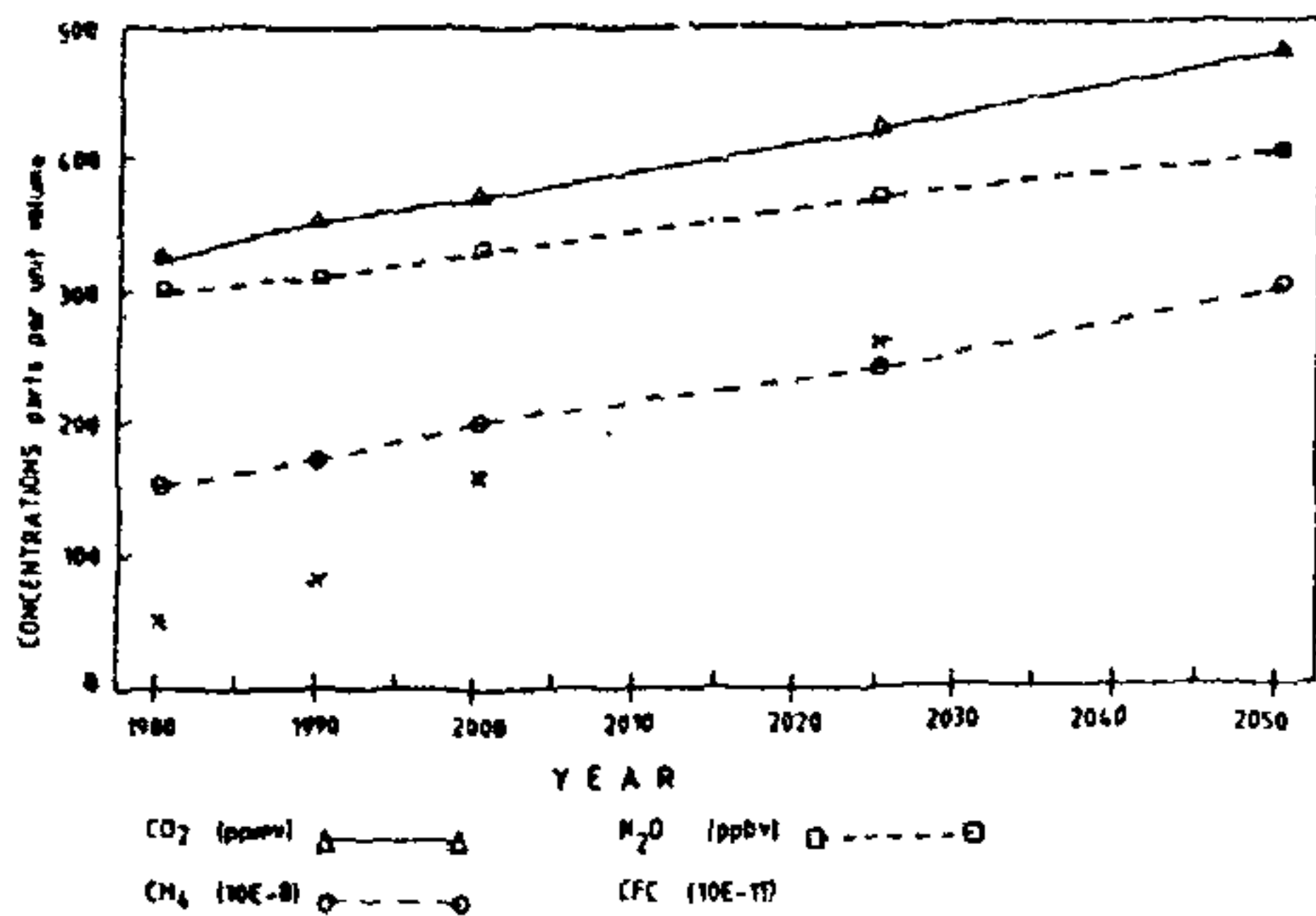
Figure 2. Growth of atmospheric concentrations of greenhouse gases based on linear extrapolation of the present rate of emission fluxes.
