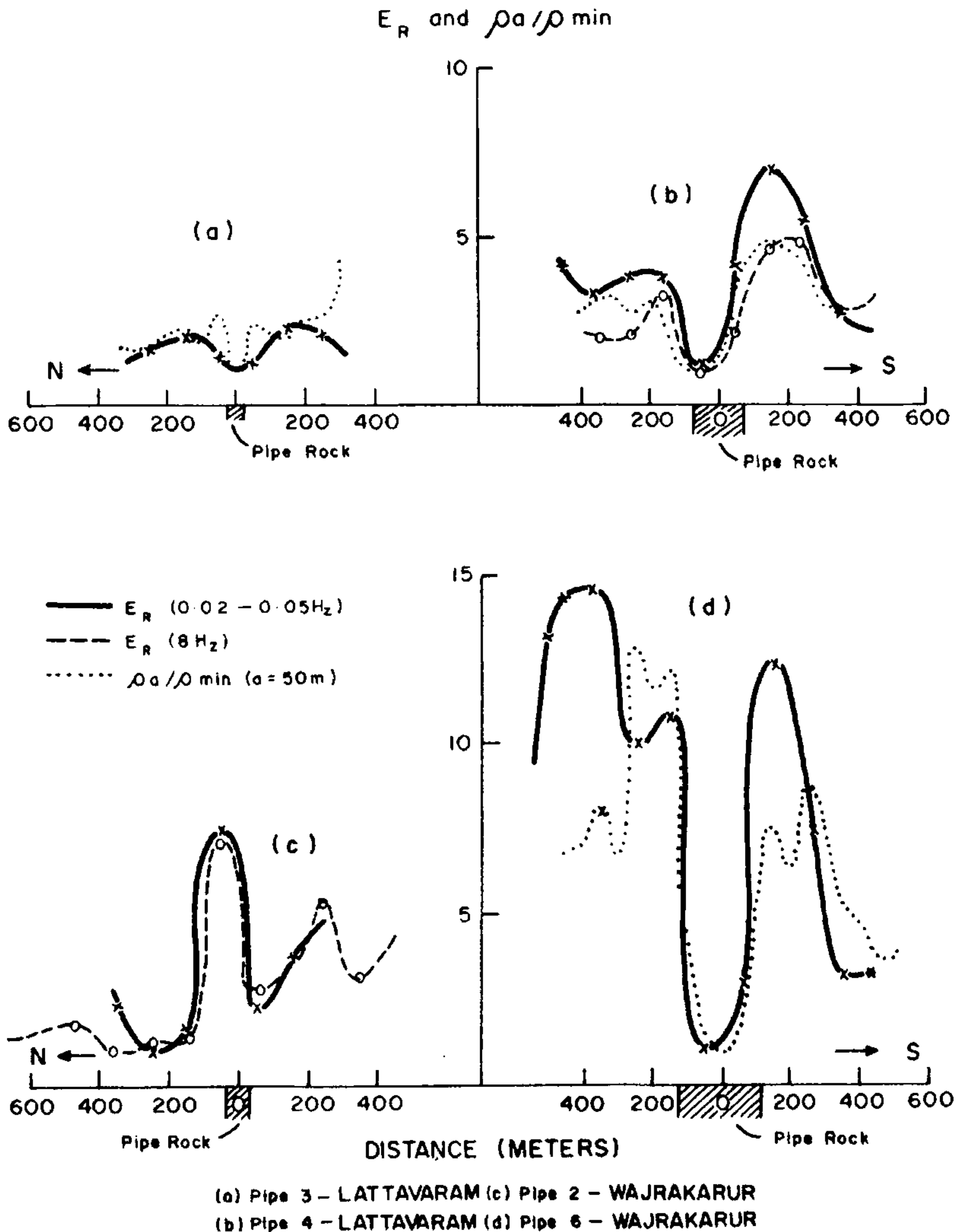
Figure 2. Telluric field ratio ( E_R ) and apparent resistivity ratio ( \rho_a / \rho_{min} ) profiles across kimberlite pipes in Wajrakarur-Lattavaram area, Andhra Pradesh, India.
