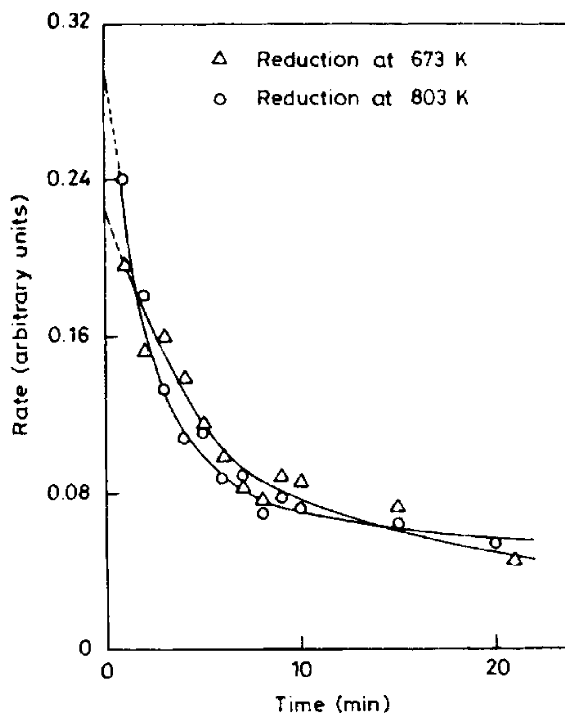
Figure 1. CO hydrogenation rate as a function of time on 15/Co/TiO 2 catalyst after LTR and after HTR.
