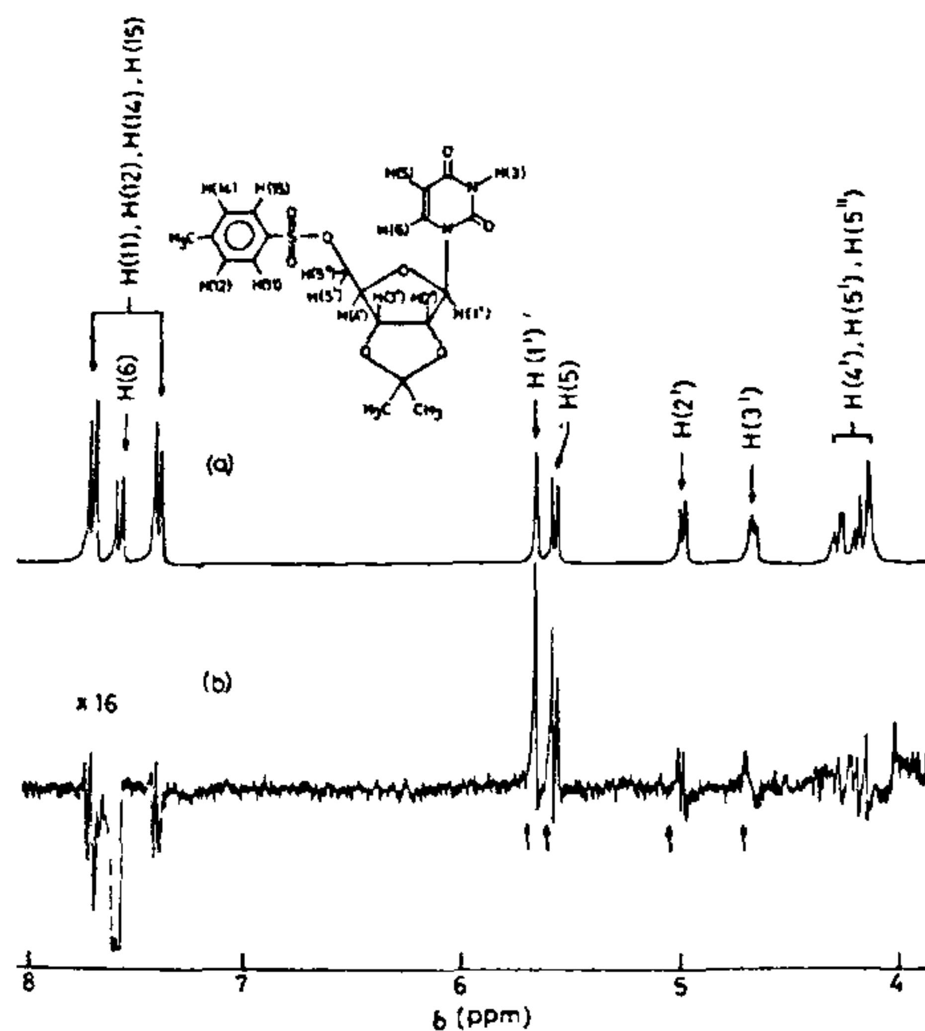
Figure 2. 270 MHz proton NMR spectra of compound I, (a) normal spectrum, (b) difference NOE spectrum magnified 16 times with respect to (a). The "normal" spectrum obtained by placing the saturating radio frequency off-resonance while keeping all other parameters identical to the on-resonance saturated spectrum case. The difference spectrum was obtained by taking the difference between the "normal" spectrum and the on-resonance saturated spectrum. The "block-averaging" subroutine of the BNC-12 computer of the Bruker WH-270 was utilized for separate collection of the two spectra and for taking the difference.
