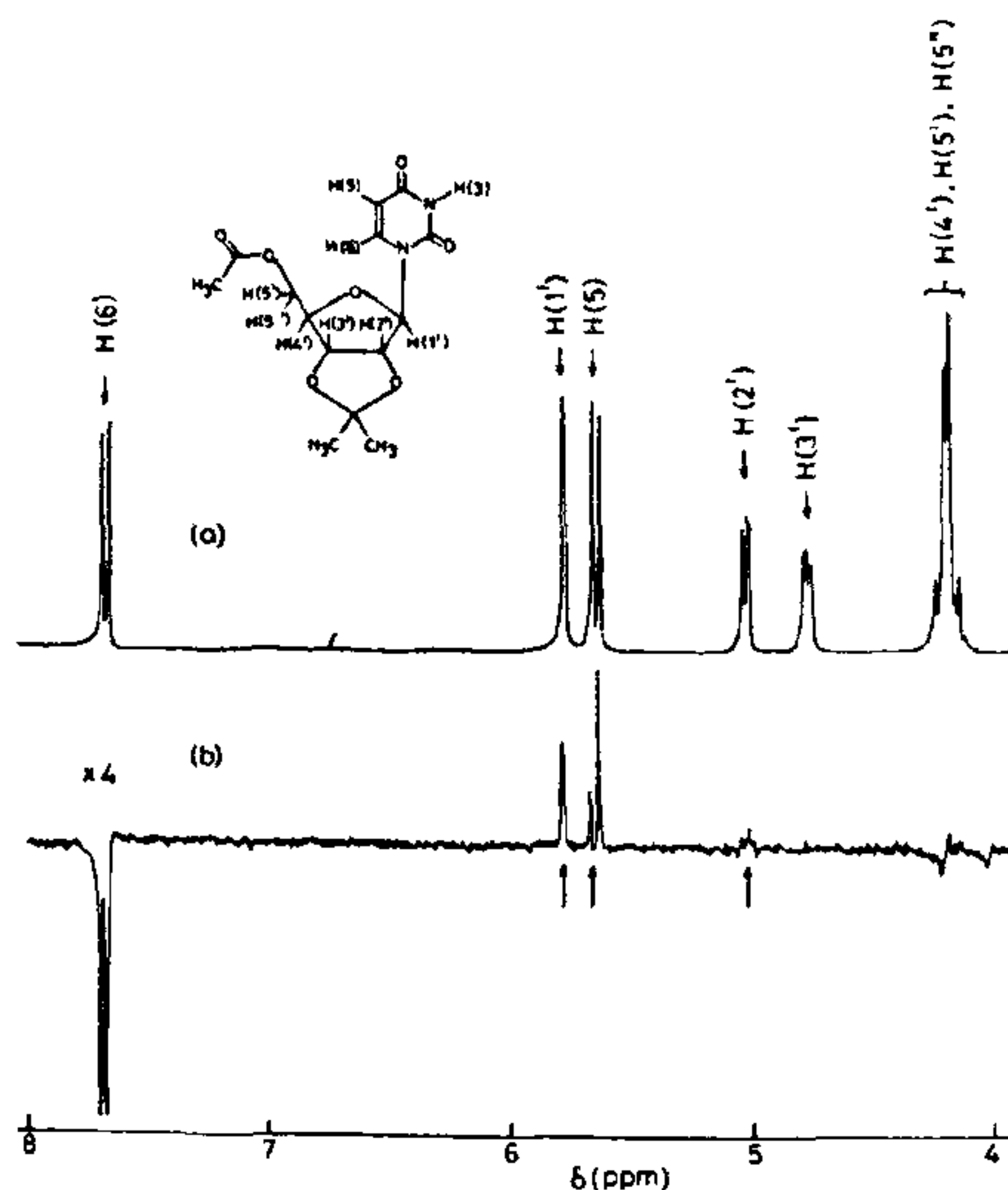
Figure 3. 270 MHz proton NMR spectra of compound II, (a) normal spectrum (b) difference NOE spectrum magnified 4 times with respect to (a). All other details same as in figure 2.
