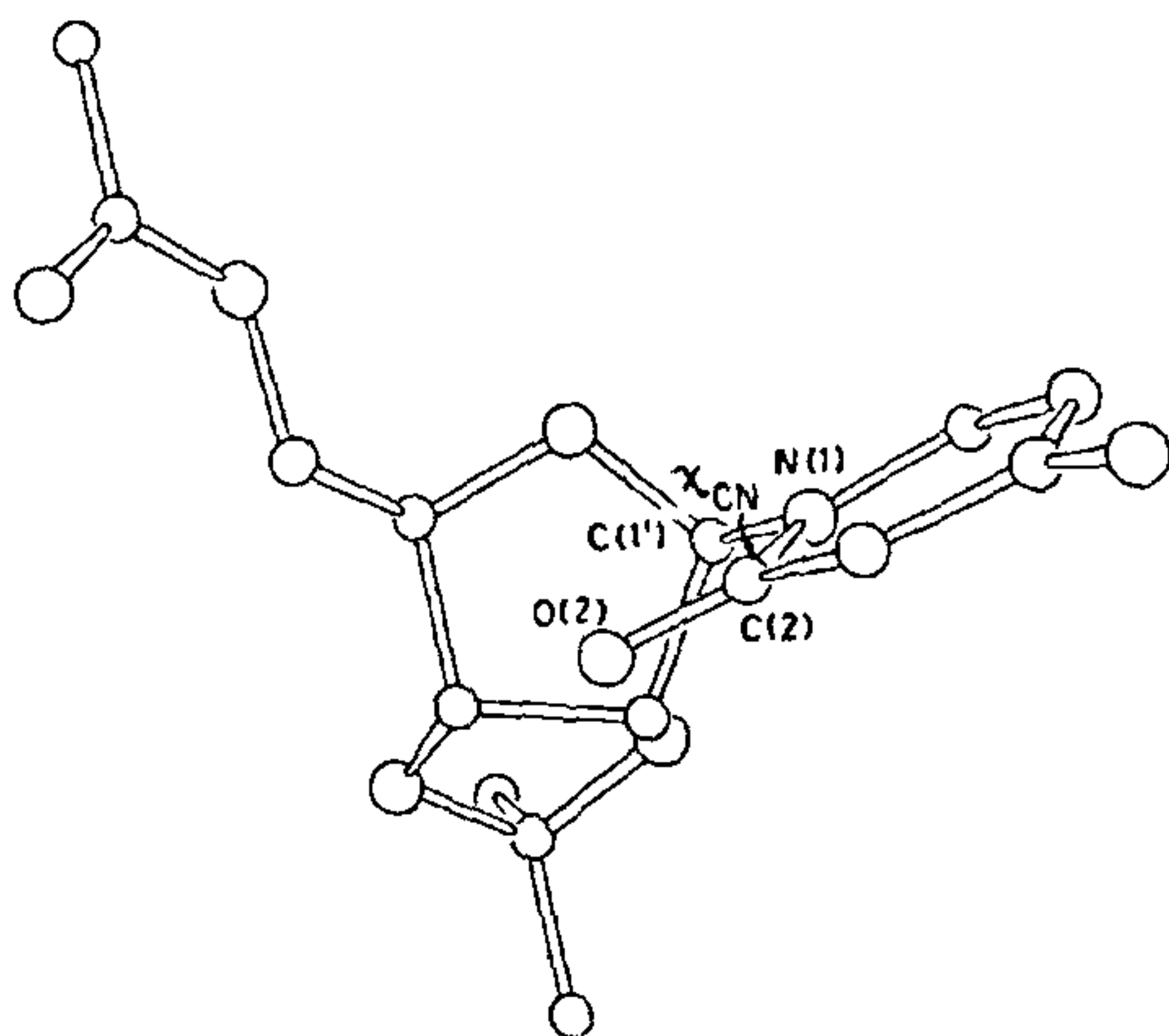
Figure 1. ORTEP drawing of II showing the syn conformation about the glycosidic bond with \chi_{CN} = -103.9^\circ , as obtained in the single crystal structure. The oxygen atom O(2) is above the ribose ring in this conformation as opposed to anti where it is away from the ring.
