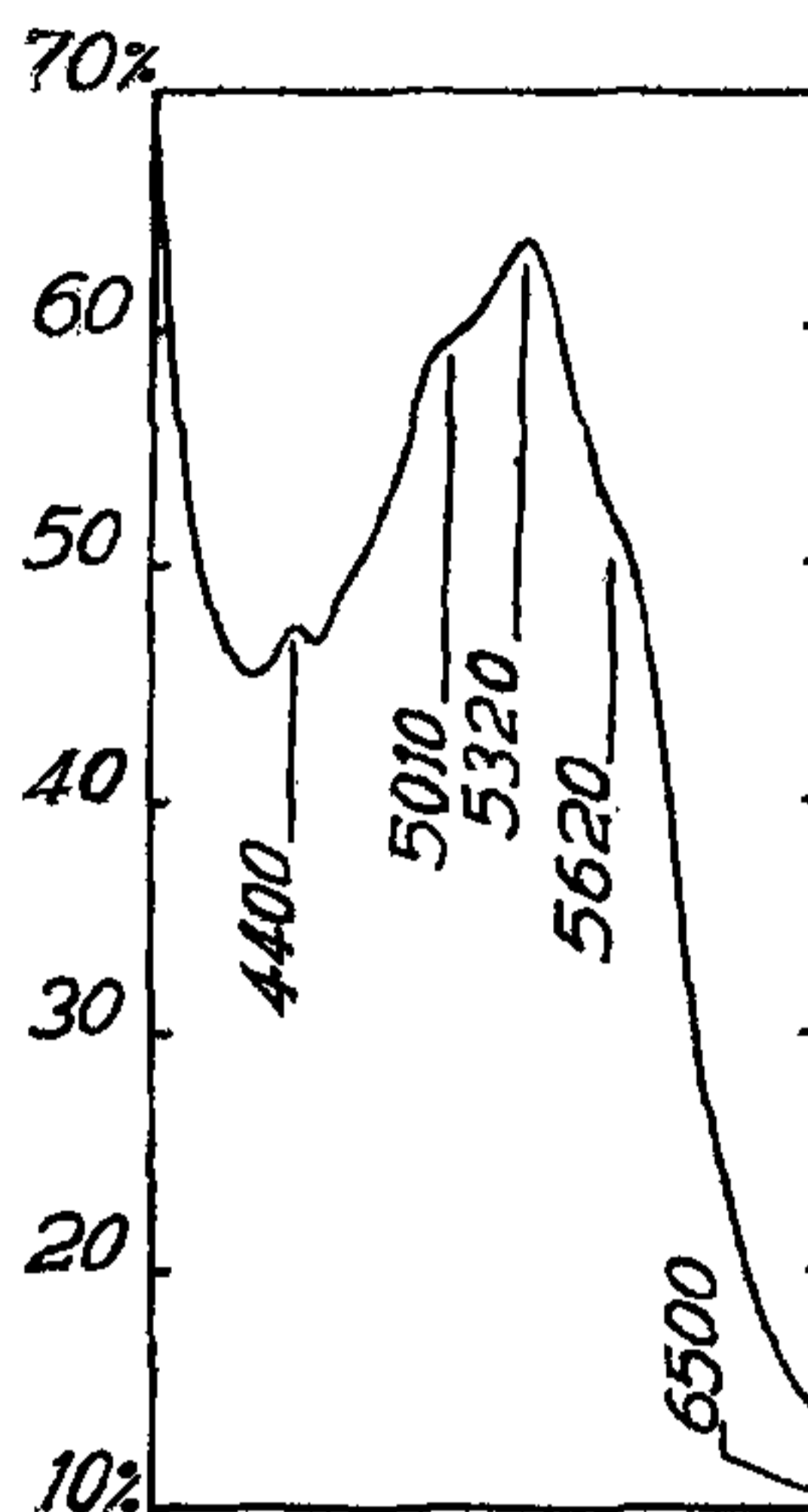
FIG. 1. Absorption by acetone extract of red Oleander
